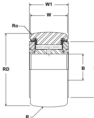
Metric Cam Yoke Roller with Crowning O.D.
